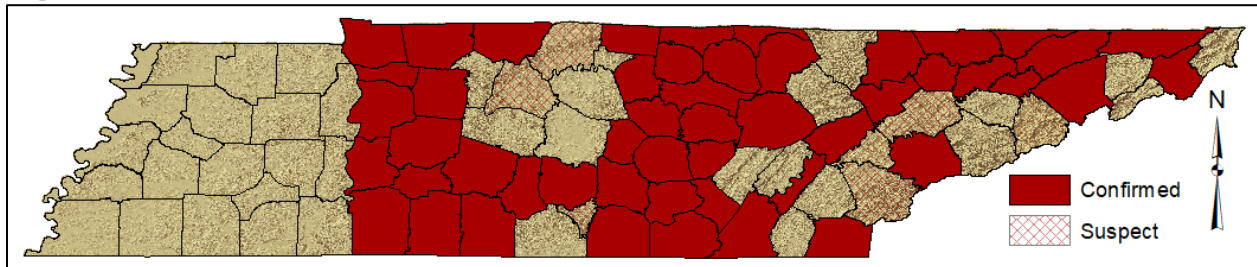
Figure 2. Most cavernous counties in Tennessee have been designated WNS confirmed and currently seven counties are WNS suspect.
