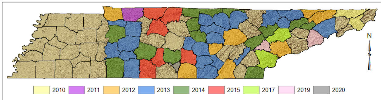
Figure 1. Progression of WNS has occurred quickly in Tennessee since being discovered in 2010. No caves were designated as WNS confirmed or suspect during the 2020-2021 monitoring period. The monitoring period includes caves surveyed from December 2020 through March 2021.
